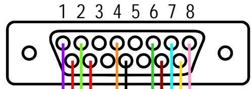
Db15 Female Plug viewed from the rear
